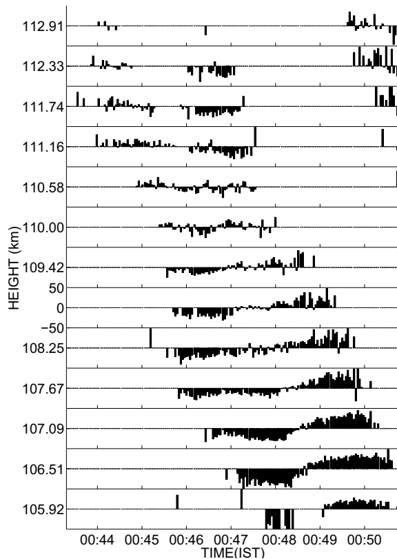
Figure 5 – Particularly clean example of a vortex-like structure seen in one QP striation with the Gadanki radar. The scale on the Y-axis between 108.25 and 109.42 km represents the line of sight Doppler velocity in \text{ms}^{-1} . From Choudhary et al. (2005).
