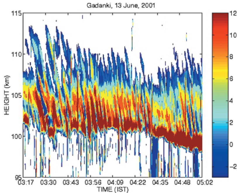
Figure 4 – Height-time-intensity plot of radar echoes showing a QP echo event observed by the Gadanki radar between 03:17 LT and 05:02 LT on June 13, 2001. Signal intensity has been plotted in eight shades of pixel coding between -3 and 12 dB.
