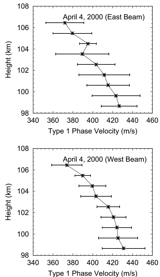
Figure 1 – Phase velocities of two-step Type I waves observed with two nearly vertical beams with the Pohnpei equatorial radar. Symbols “x” connected by the line are the averages obtained with the data samples. More details on the data can be found in St.-Maurice et al. (2003).
