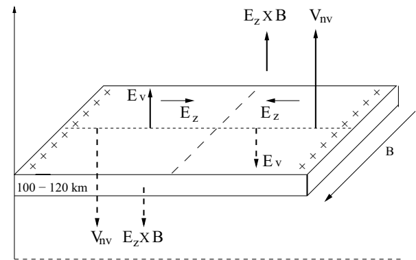
Figure 6 – Cartoon illustrating the basic reason why the vertical wind structure of a Kelvin-Helmholtz billow will be detected by an upward looking radar. From St.-Maurice & Choudhary (2006).
