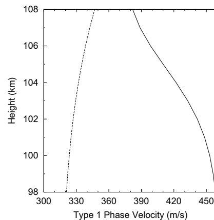
Figure 2 – Full line: phase velocity computed for the non-isothermal threshold speed. Broken line: isothermal ion-acoustic speed. Adapted from St.-Maurice et al. (2003).
