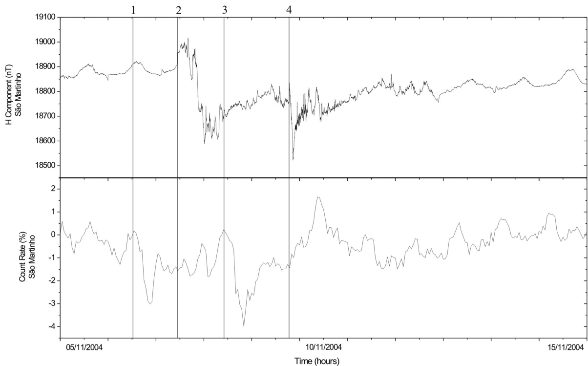
Figure 2 – Variations in H Component of Earth's Magnetic Field and Count Rate of the Muon Scintillator Telescope for the period of 5-15 November 2004.
